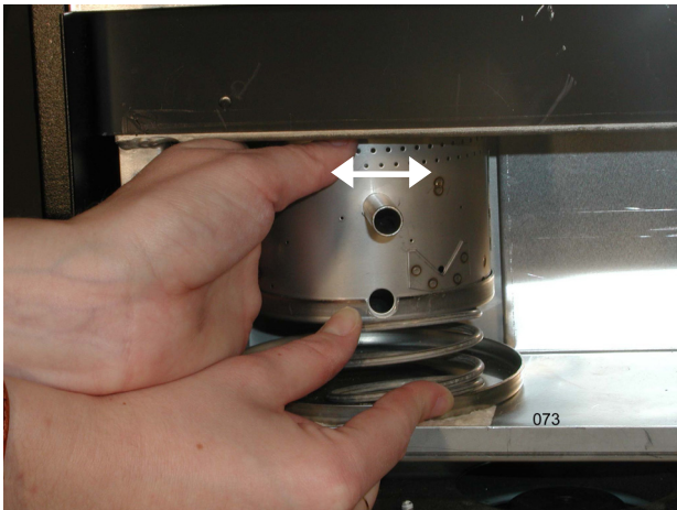
Figur 15: Brännarens montering.
