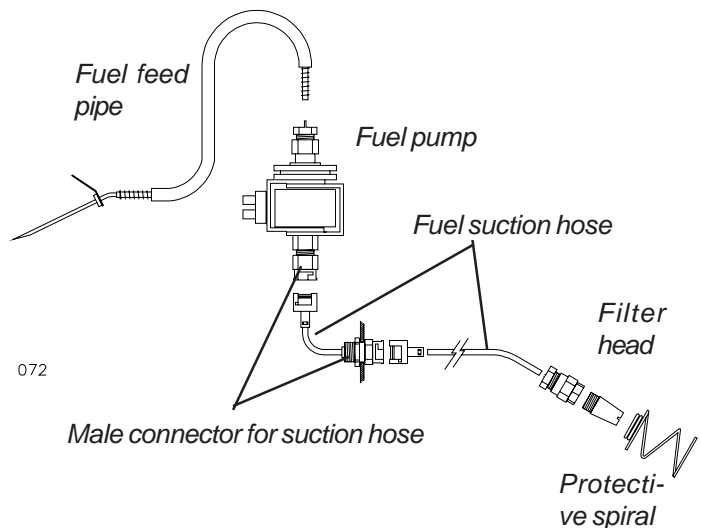
Fig. 16: Fuel system parts.
