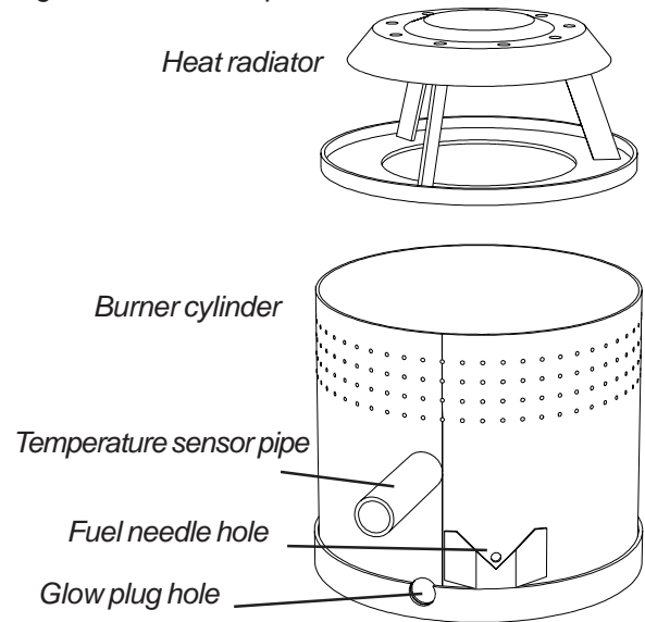
Fig. 13: Detaching the heat radiator.
