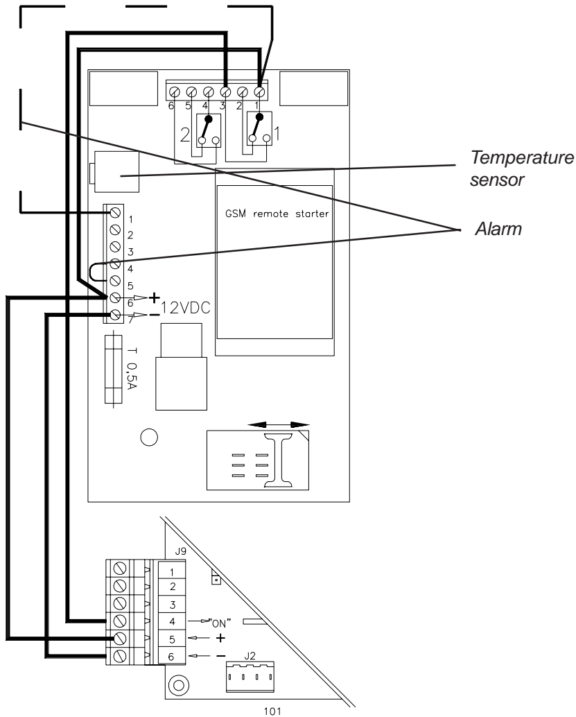
Fig. 19. Connecting a solenoid valve to the heater.
