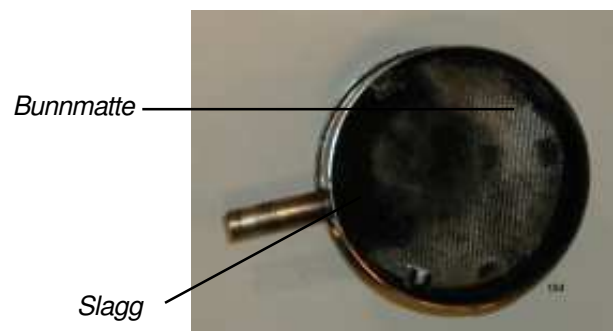
Bilde 14: Brennersylinder.
