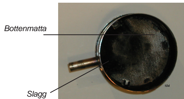
Figur 14: Brännarcylinder.
