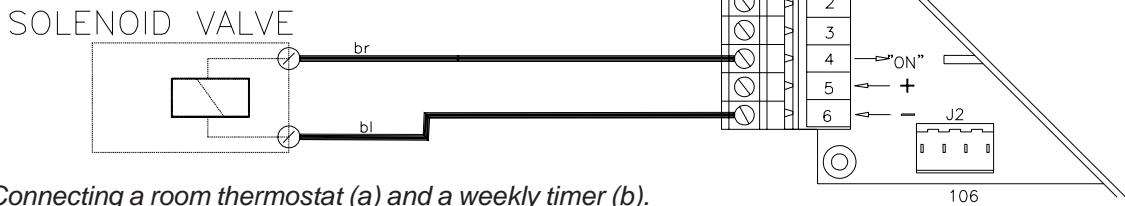
Fig. 20. Connecting a room thermostat (a) and a weekly timer (b).
